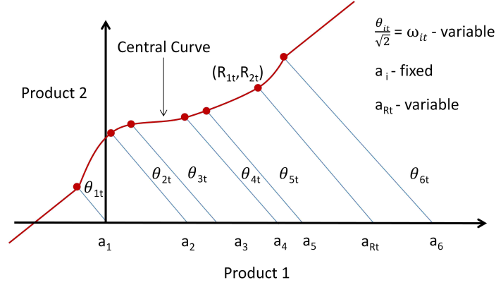
Figure 3.1: Spline Function
